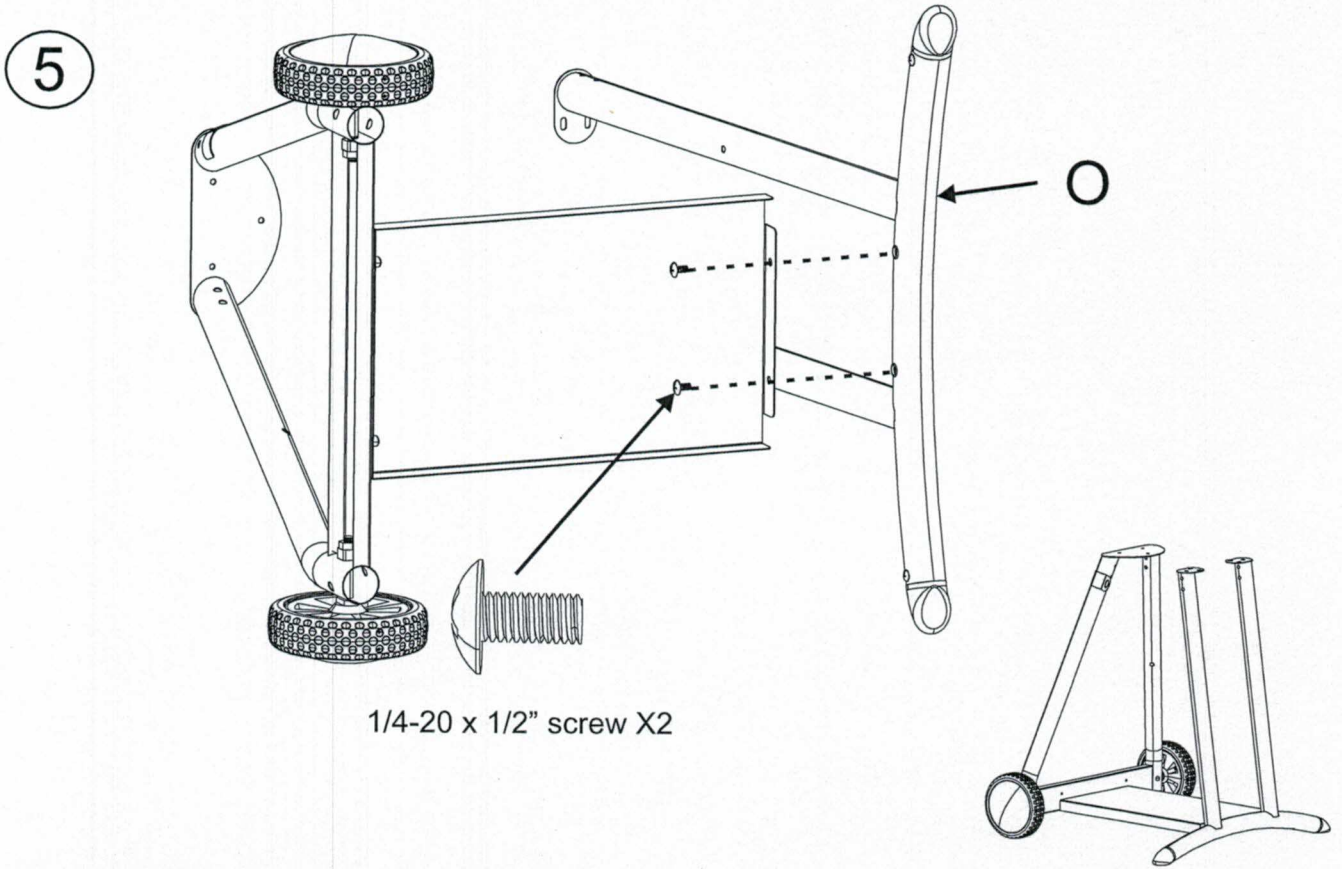
Final assembly
