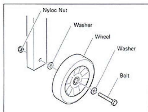
WHEEL ASSEMBLY
