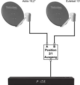
Beispiel 1: 2 Satelliten (Single-LNBs) Astra 19,2° Eutelsat 13°
