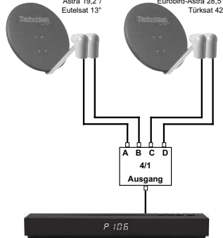
Beispiel 2: 4 Satelliten (Single-LNBs) Astra 19,2°/ Eutelsat 13° Eurobird-Astra 28,5°/ Türksat 42°
