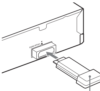
Transceiver wireless
