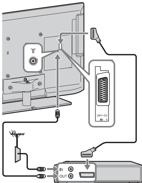
Set-Top-Box/Recorder (z. B. DVD-Recorder)
