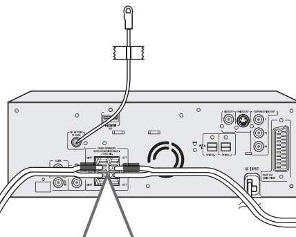
Antenna FM
